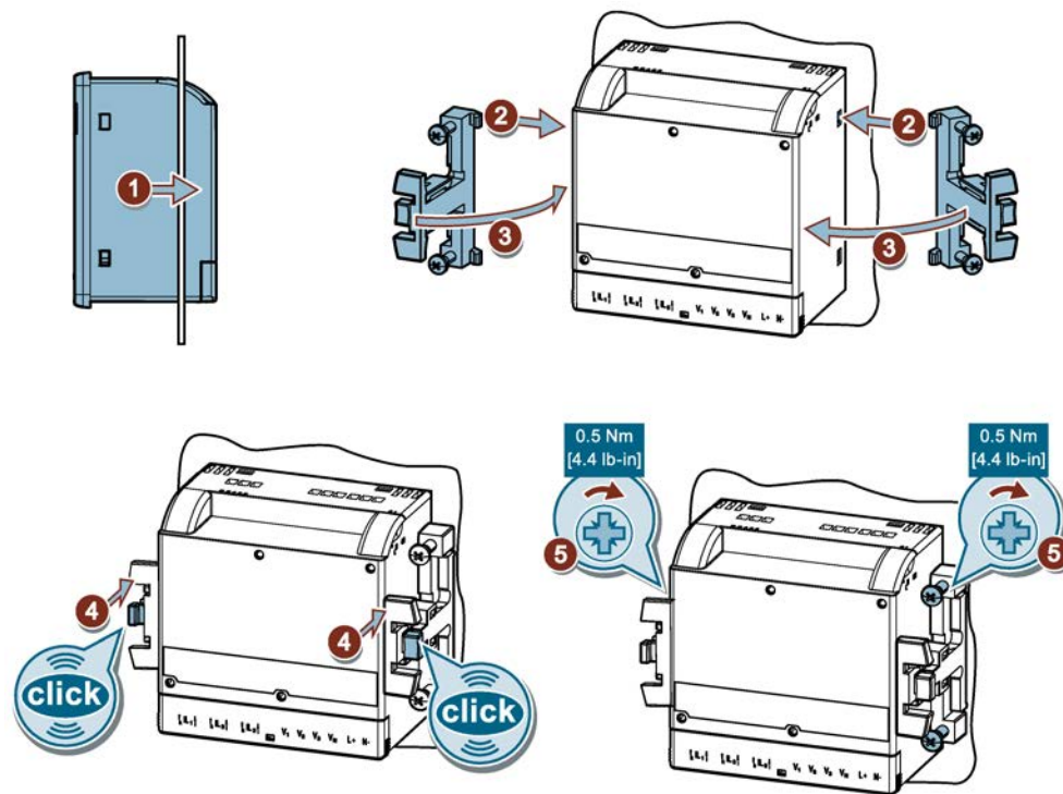
Figure 3-2 Mounting
