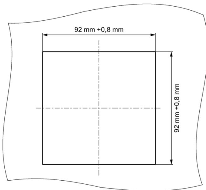
Figure 11-1 Panel cutout
