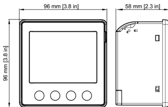
Figure 11-2 Frame dimensions
