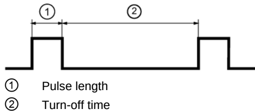
Figure 2-7 Pulse length and turn-off time
