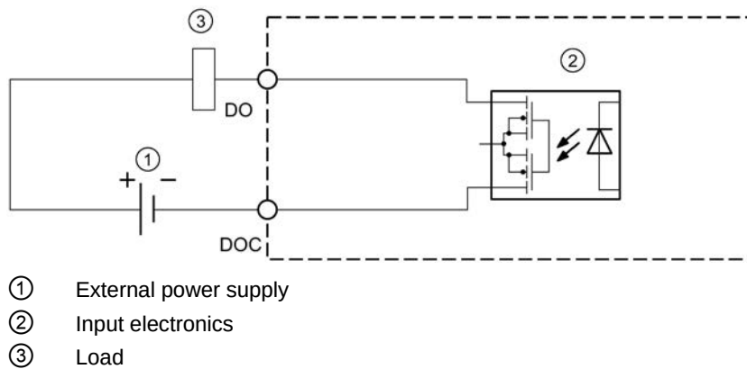
Figure 2-5 Block diagram: Digital outputs
