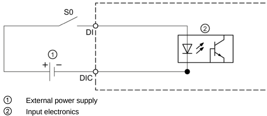
Figure 2-3 Block diagram: Digital inputs
